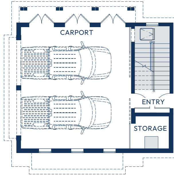
FIRST LEVEL
