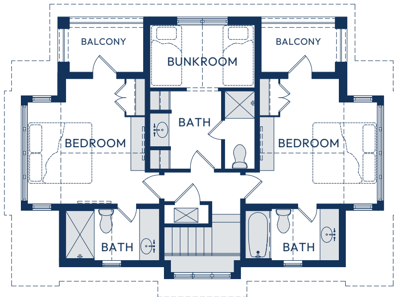
THIRD LEVEL
