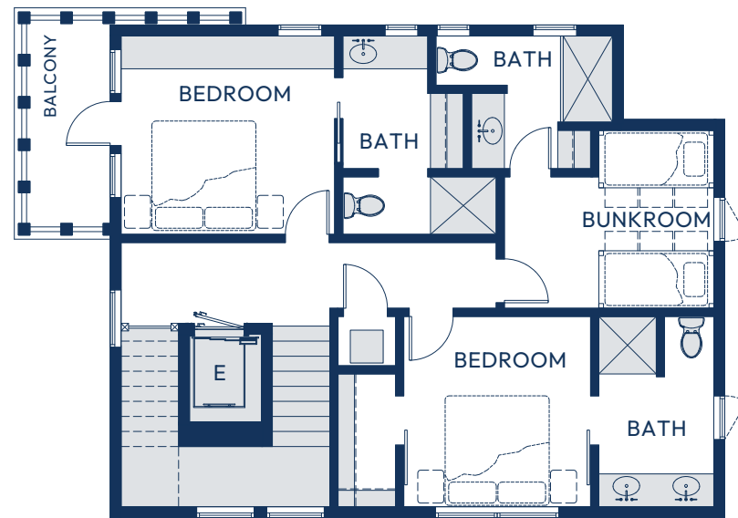
THIRD LEVEL
